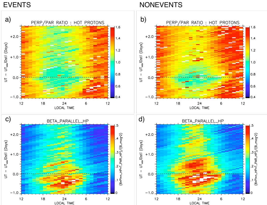
Figure 4.5 (a and b) Temperature anisotropy and (c and d) plasma beta \beta_{||h} for hot proton populations. These two parameters are the main components in the calculation of the observational EMIC growth parameter \Sigma_h .
