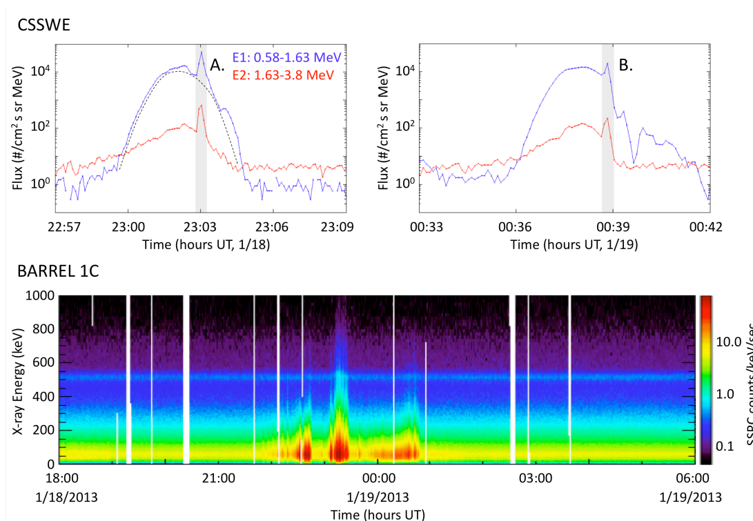
Figure 7.1 (top) Measurements from the CSSWE CubeSat and (bottom) BARREL balloon 1C during a precipitation event on 18–19 January 2013. CSSWE measures two precipitation bands (labeled A and B and indicated by the shaded grey regions) on two consecutive passes through the outer belt. The dashed black line suggests the background trapped and bounce loss cone flux upon which the precipitation bands are superimposed. (bottom) X-ray spectra from balloon 1C are shown from 18:00 UT 18 January through 06:00 UT 19 January. During this time, three main precipitation events are measured by the balloon, the second two showing X-rays of energies >0.5 MeV. No background subtraction has been applied here to either the BARREL or CSSWE measurements.
