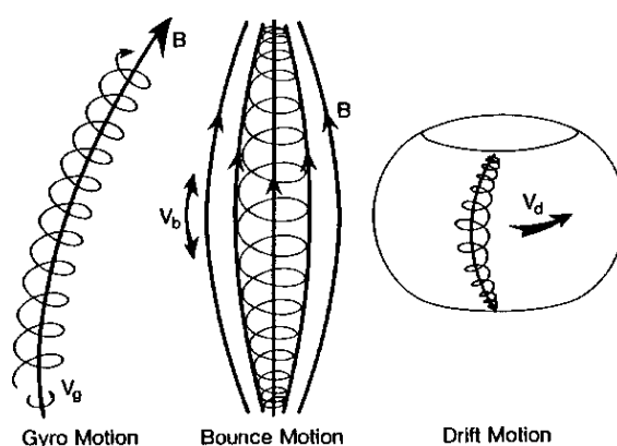
Figure 2.5 The three characteristic motions of a charged particle in a dipole magnetic field. An electron (proton) will gyrate about the field line in a right (left) hand sense (depicted on the far left). A field-aligned gradient of the magnetic field causes a particle’s parallel velocity to decrease as it moves to regions of higher field strength, until a point termed the “mirror point” when it reverses and returns back along the field line. Motion between two mirror points creates the bounce motion depicted in the middle panel. Finally, field gradient and curvature effects cause electrons (protons) to drift eastward (westward) about Earth as they gyrate and bounce (depicted on the far right). (From Kivelson and Russell, 1995)
