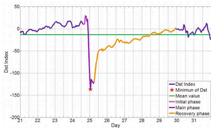
Figure 2.7 Dst index during a geomagnetic storm occurring on Day 25. The three primary storm phases are marked in different colors, pink, purple, and yellow. (From Sarachaga et al., 2014)
