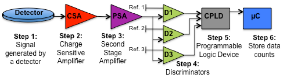
Figure 6.3 Instrument electronics block diagram. (From Blum and Schiller , 2012)
