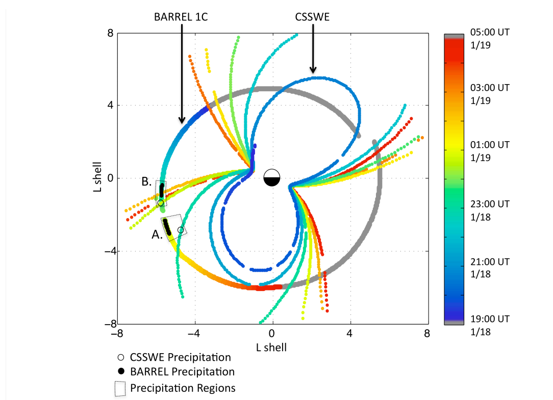
Figure 7.3 The location of CSSWE and balloon 1C mapped to the magnetic equatorial plane, with local noon at the top. Universal time of the locations is shown on the color bar. The balloon drifts across the dusk sector at a fairly constant L \sim 5.5-6 , while the CubeSat cuts across this track every roughly 90 min. The locations of the precipitation bands, as measured by CSSWE, are indicated by the open black circles. The tracks of solid black circles indicate when balloon 1C measures >0.5\text{MeV} X-rays due to precipitating electrons. The dotted boxes outline the two precipitation regions as determined from the conjunctive measurements, (exact dimensions of these regions are listed in Table 7.1).
