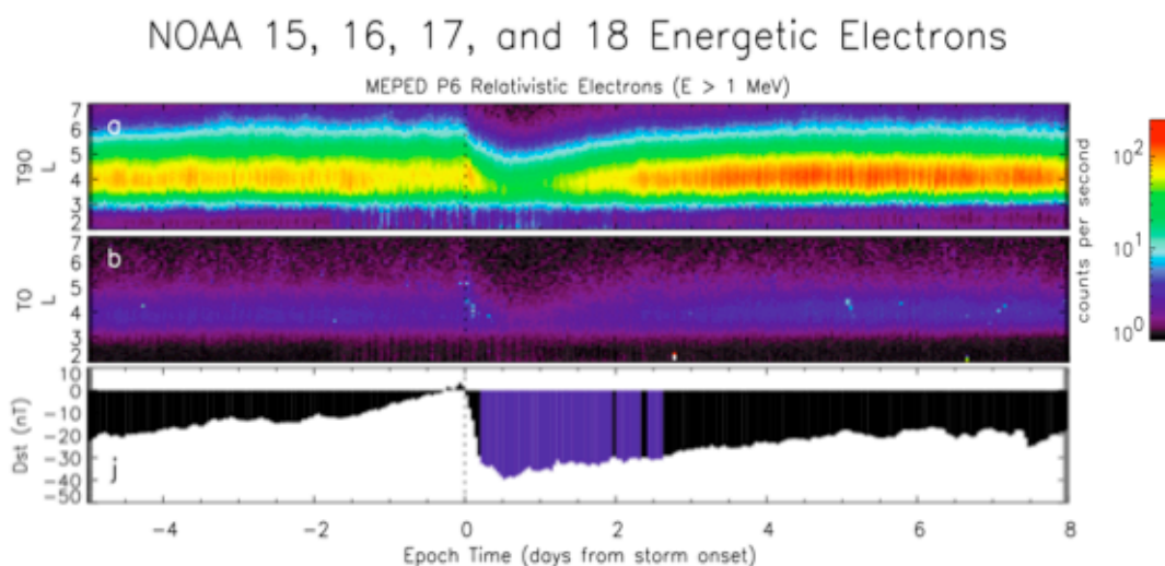
Figure 5.12 Superposed POES energetic electrons and Dst index during 42 HSS-driven storms. (Adapted from Meredith et al. , 2011)
