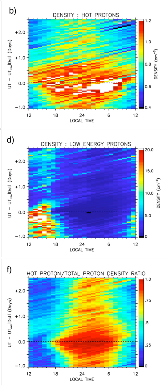
Figure 4.4 (a and b) Hot proton density n_h , (c and d) cold proton density n_c , and (e and f) density ratio n_h/n_e across local and epoch times for events and nonevents. Density ratio n_h/n_e is lowest in the region from approximately noon to dusk, where the cold dense plume is located.
