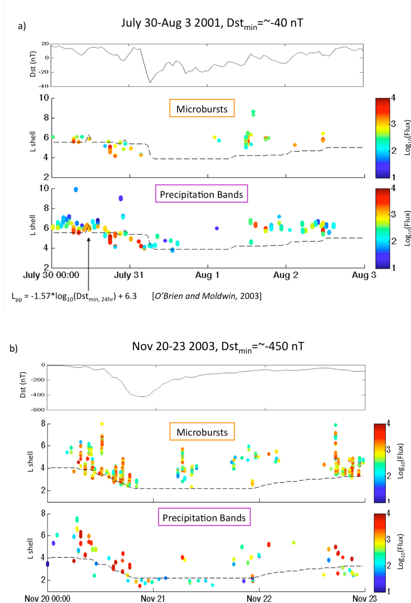
Figure 5.11 Dst (top panel), microburst magnitude (middle), and precipitation band magnitude (bottom) across L shell and time during two geomagnetic storms – a small storm in 2001 (a) and much larger superstorm in Nov 2003 (b). A model for the plasmapause location is plotted with the dashed black line.
